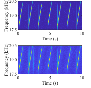
Fig. 2: Example signals: water (top) vs tortilla (bottom).
